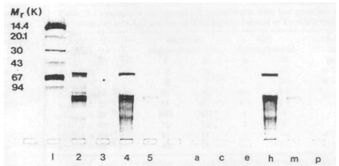
Fig. 2 Electrophoresis (polyacrylamide 7-15%, bands revealed by silver staining): samples numbered 1 to 5 are standards for the blind experiments a, c, e, h, m, p. Lane 1. Molecular weight standards for electrophoresis; lane 2, monoclonal IgG added with human serum albumin; lane 3. Tyrode's buffer without human serum albumin; lane 4. 1 \times 10^2 anti-IgE dilution; lane 5. 1 \times 10^3 dilution. Samples tested: a and c, buffer; e, 1 \times 10^{36} anti-IgE dilution; h, 1 \times 10^2 anti-IgE dilution; m, 1 \times 10^3 anti-IgE dilution; p, 1 \times 10^{35} anti-IgE dilution.
